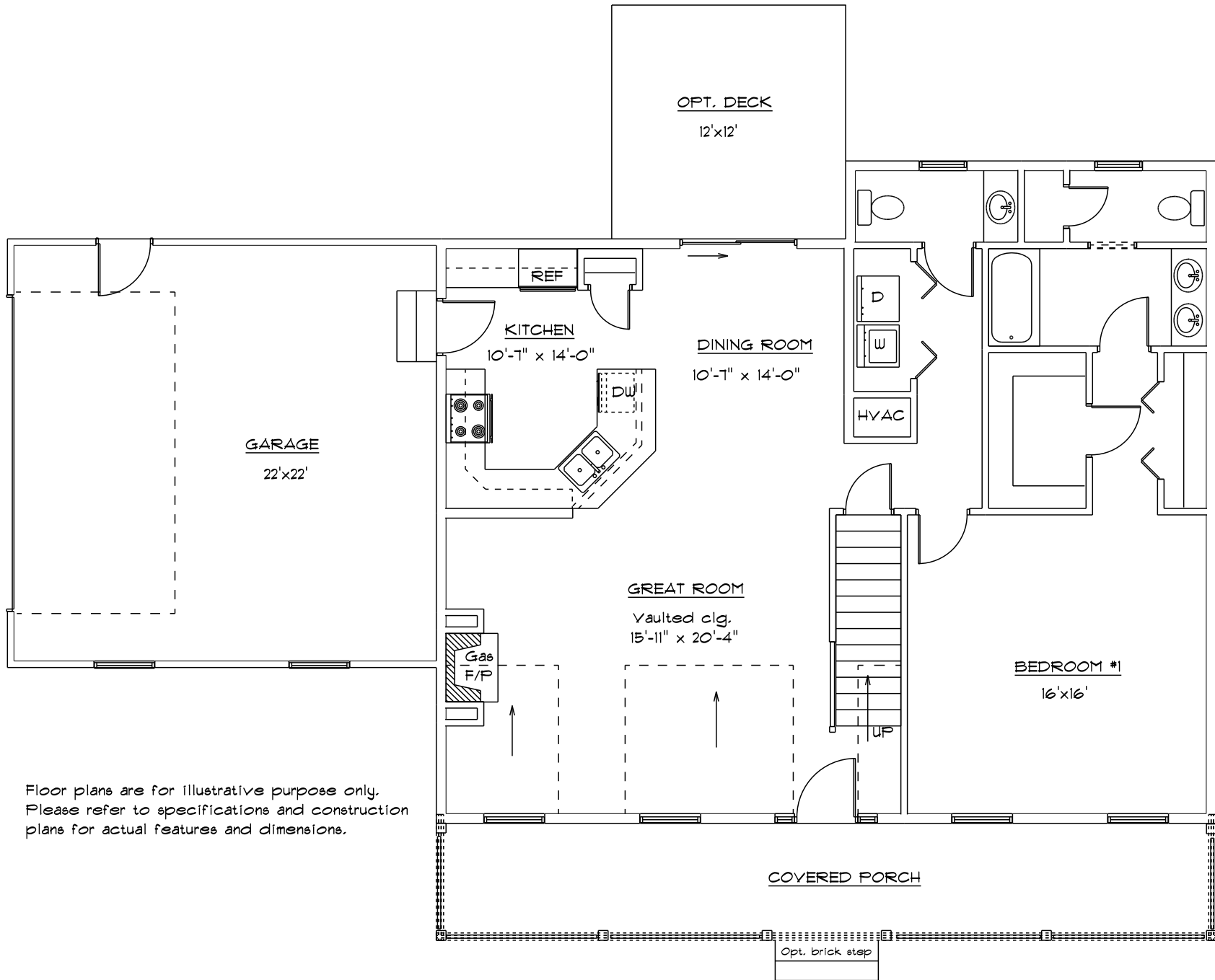
The Glendale First Floor Plan
