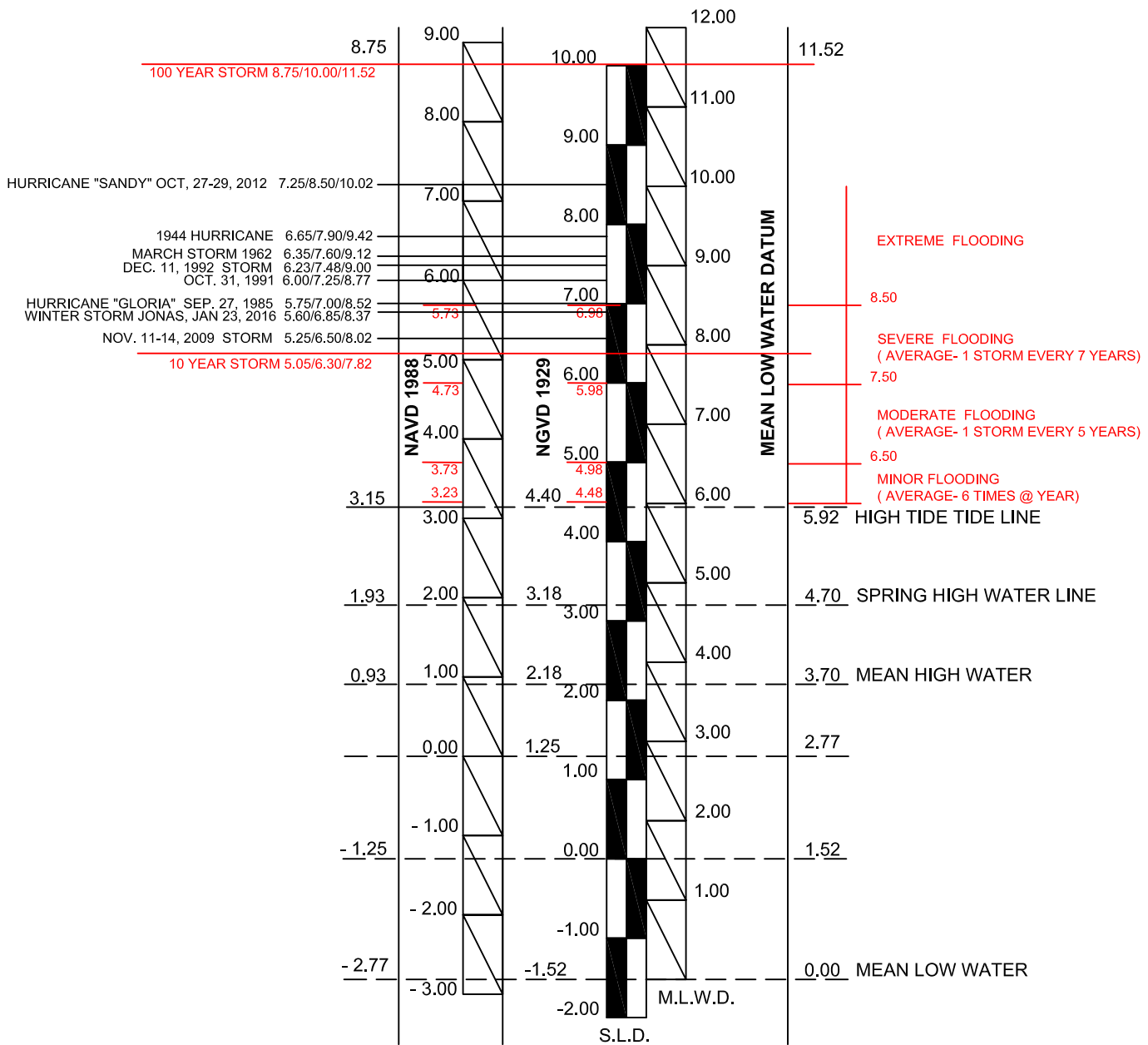
TIDE HEIGHTS RELATIVE TO N.A.V.D. 1988, N.G.V.D. 1929 & M.L.W. DATUM OCEAN CITY, NJ HISTORIC TIDE INFORMATION FROM 520 BAY AVENUE TIDE STATION AND WALLACE HARDWARE STORE
