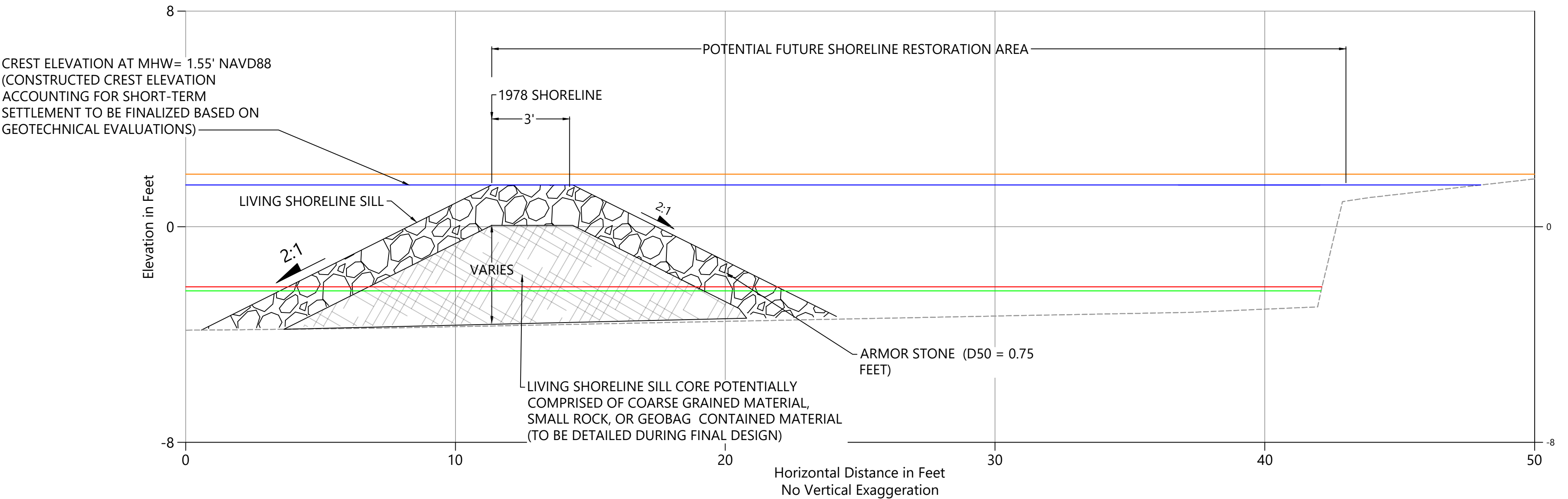
LIVING SHORE CROSS SECTION
