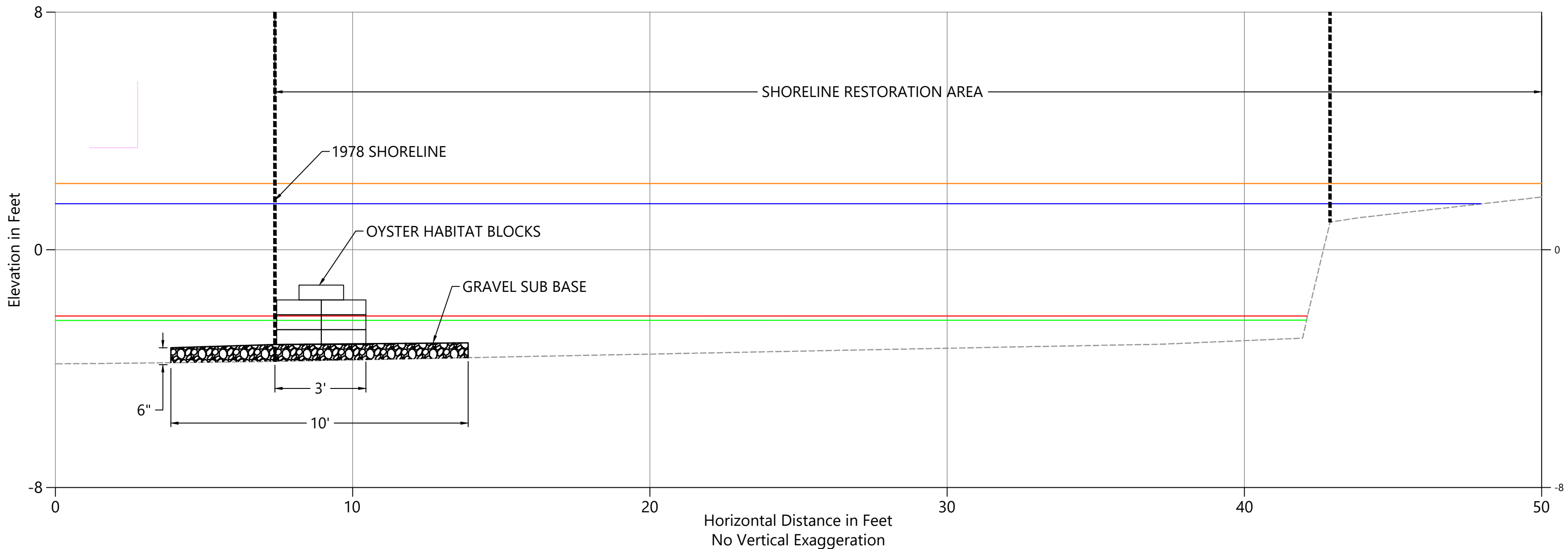
LIVING SHORE CROSS SECTION
