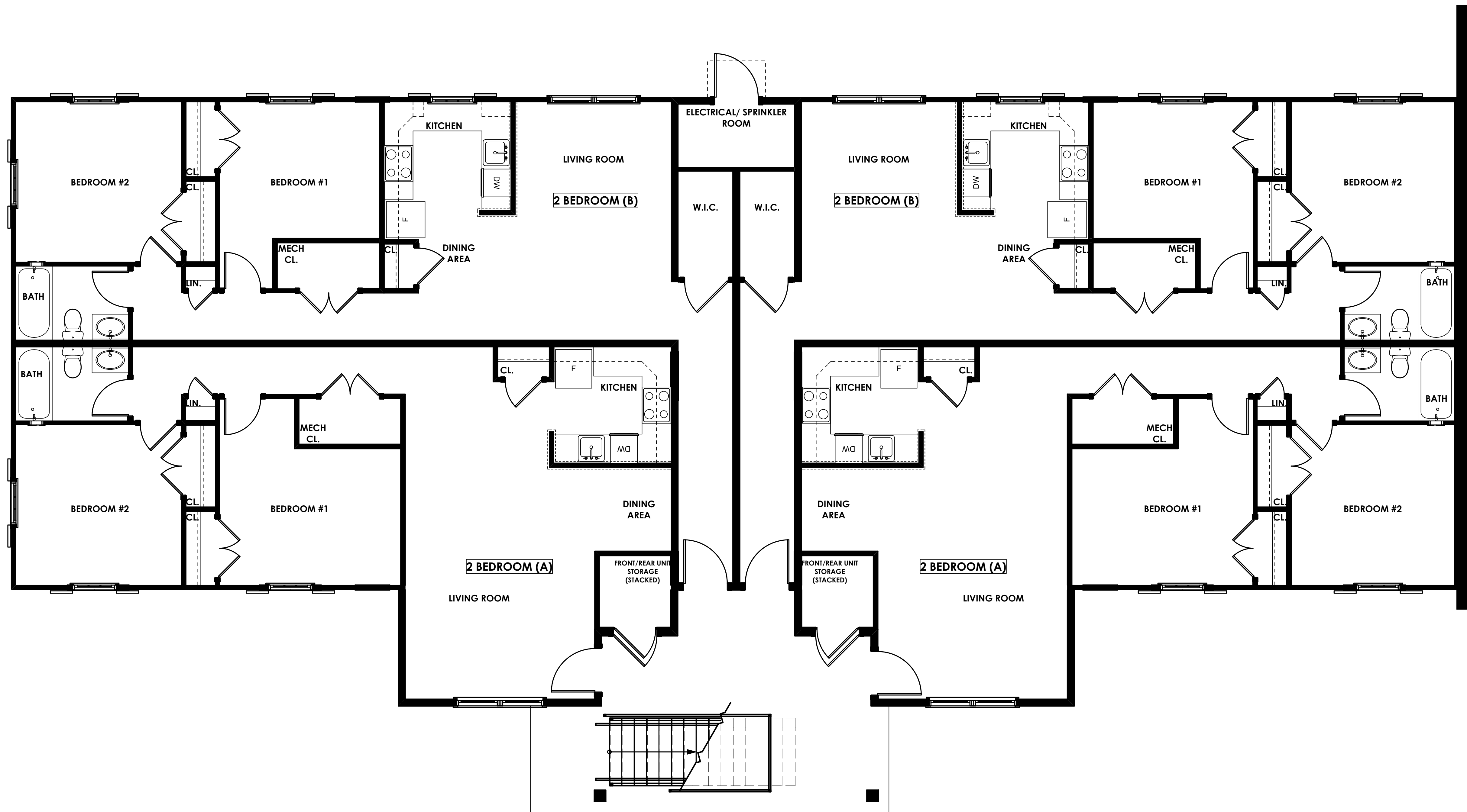
STANDARD 8-PACK FIRST FLOOR PLAN
