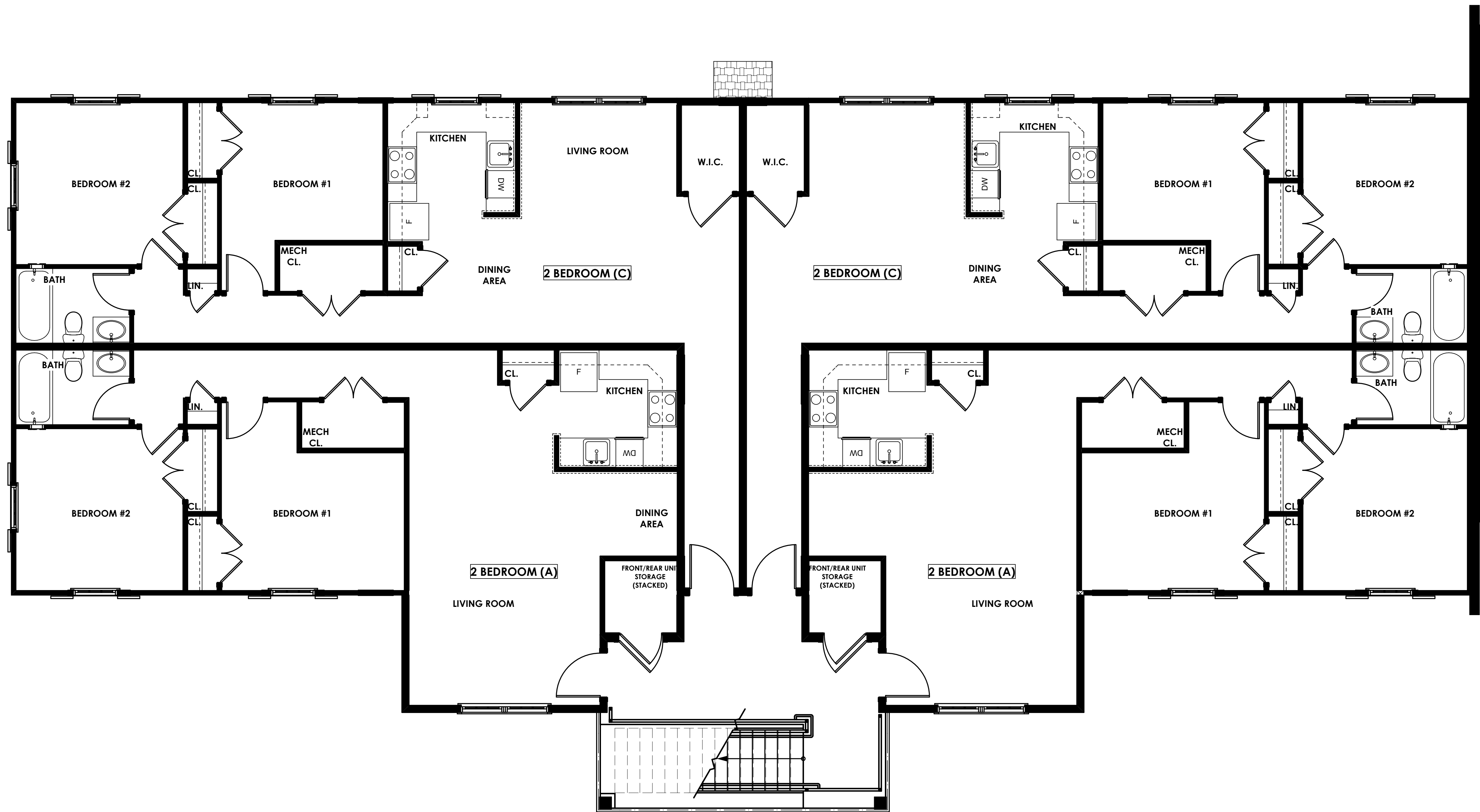
STANDARD 8-PACK SECOND FLOOR PLAN
