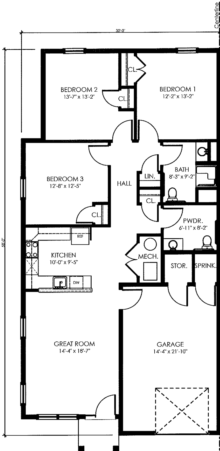
Floor Plan Typical 3 Bedroom HC Unit
