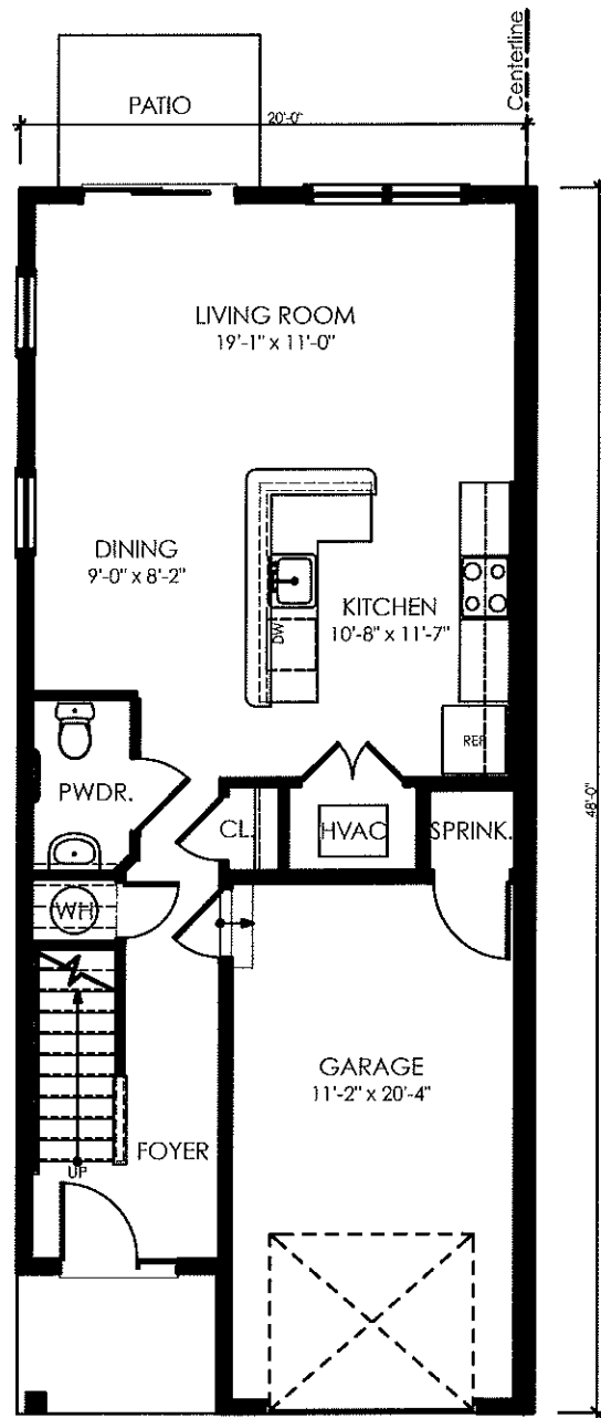
First Floor Plan Typical 3 Bedroom 2-Story Unit
