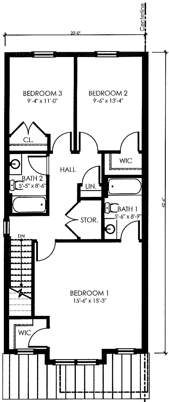
Second Floor Plan Typical 3 Bedroom 2-Story Unit
