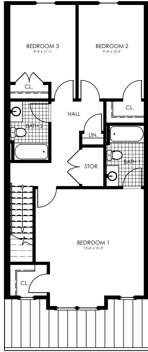
SECOND FLOOR
