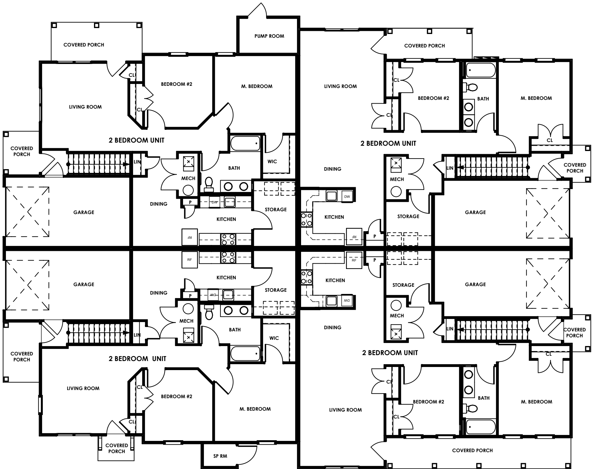
TYPICAL BUILDING PLAN - FIRST FLOOR
