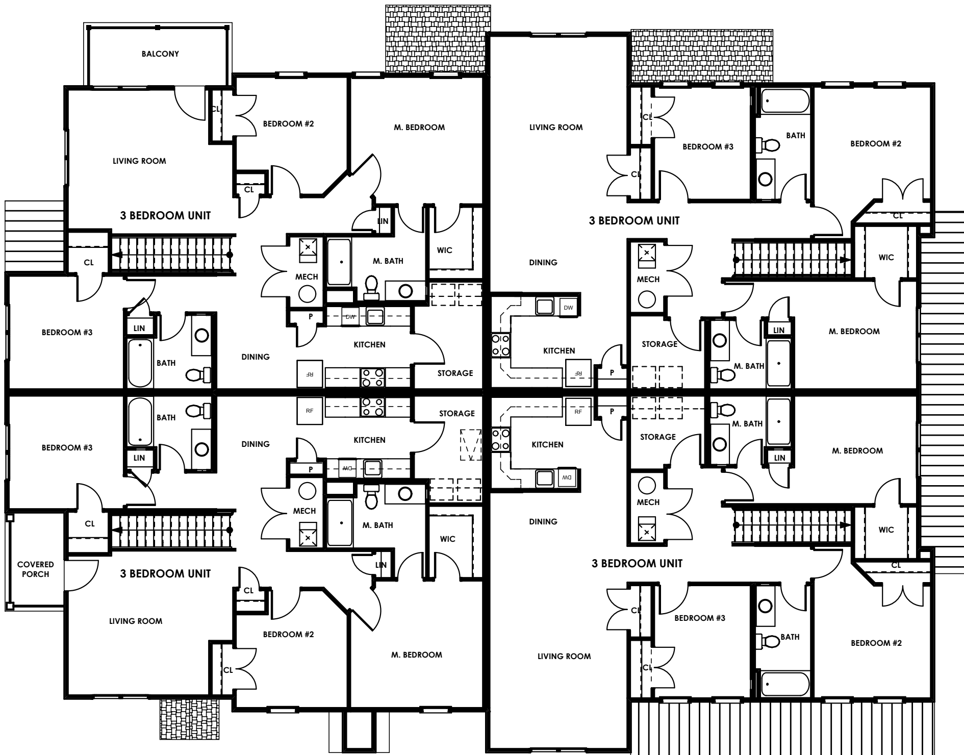
TYPICAL BUILDING PLAN - SECOND FLOOR
