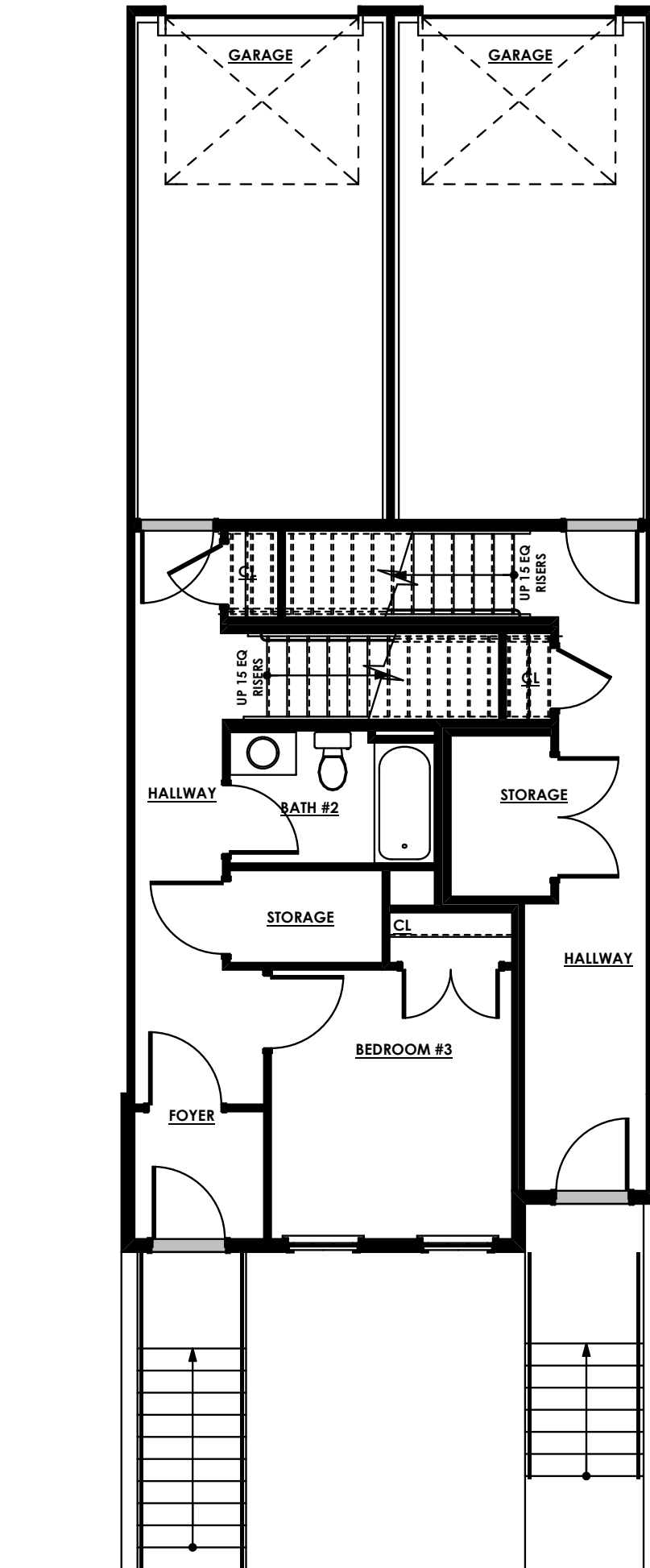
FIRST FLOOR - TWO UNITS
