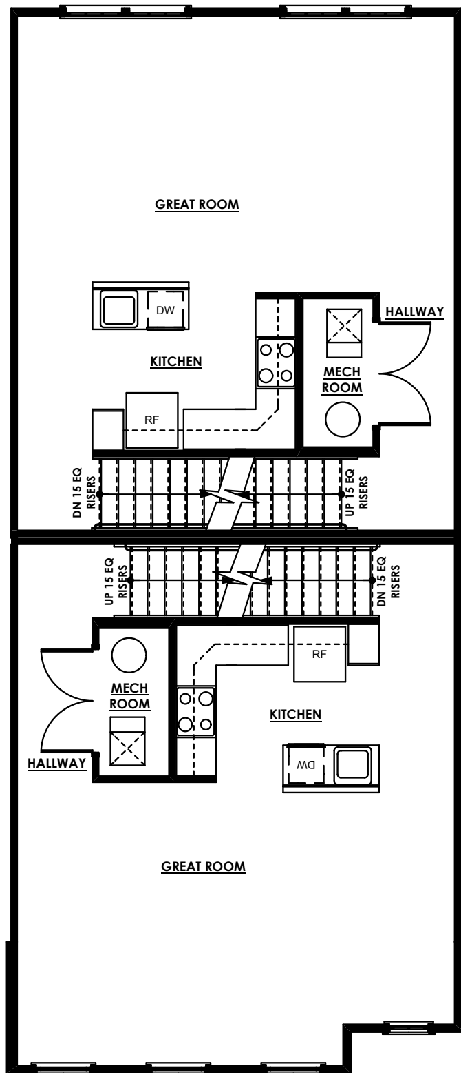
SECOND FLOOR - TWO UNITS
