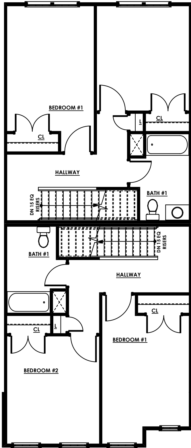
THIRD FLOOR - TWO UNITS
