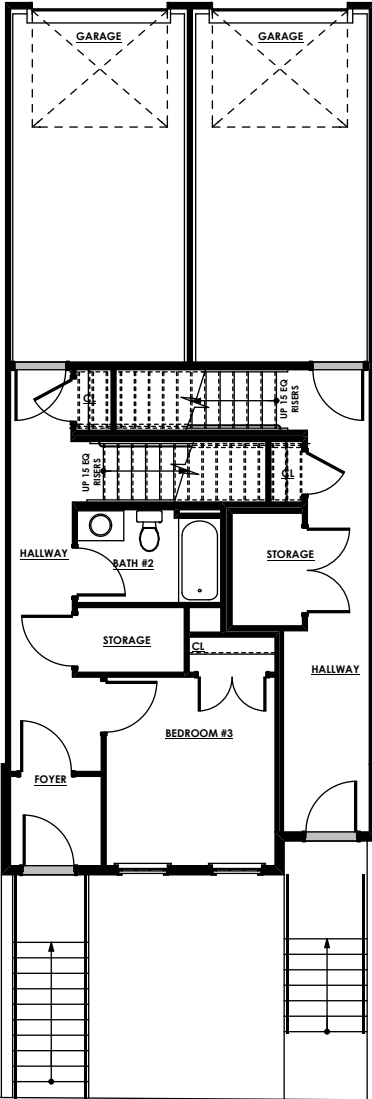
FIRST FLOOR - TWO UNITS
