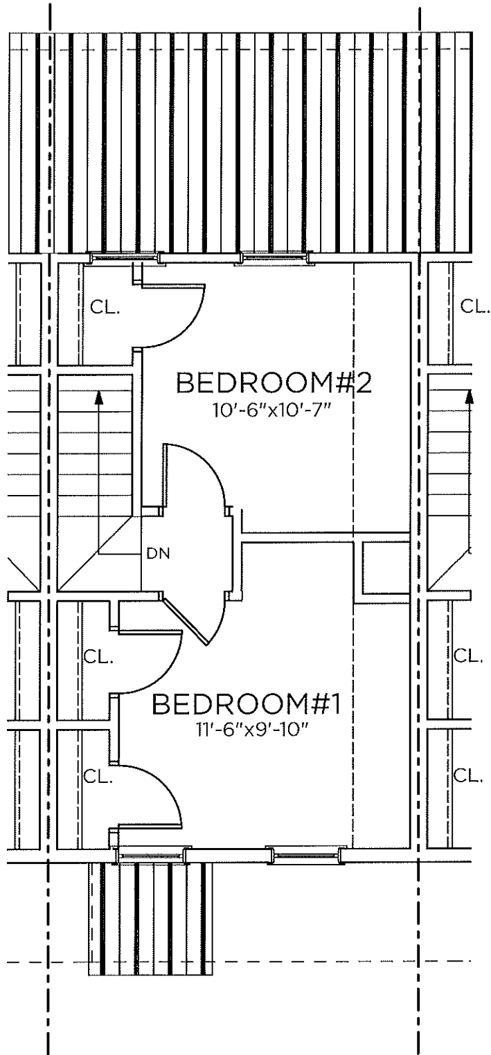
SECOND FLOOR PLAN HIGH STEPS APARTMENT
